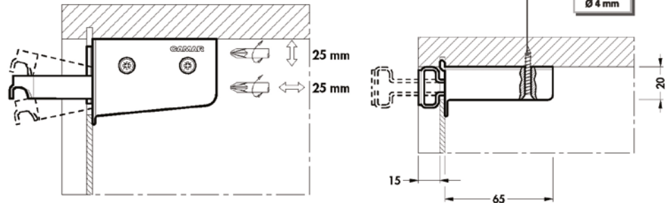
875-Z1 Rails
