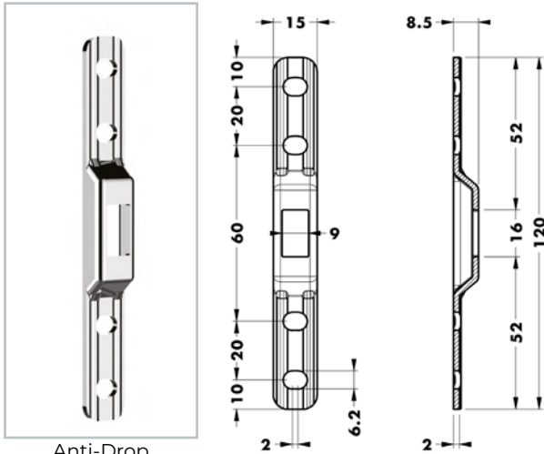
Anti-Drop Wall Plate
