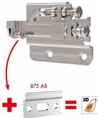
Screw Mount
