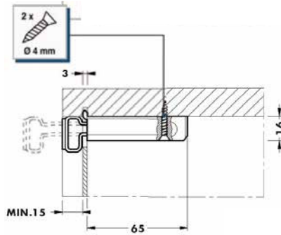
Screw Mount
