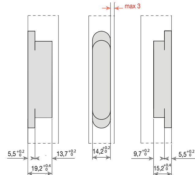
Slot measurement
