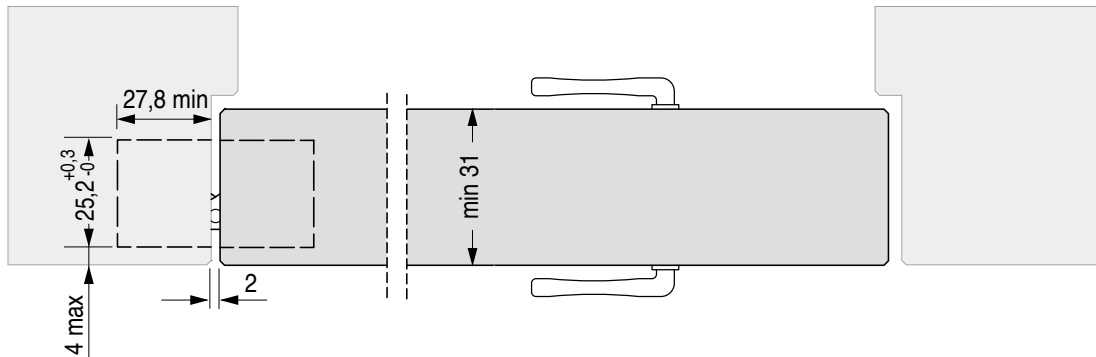
Door cross-section
