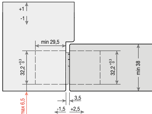
Unrebutted flush door cross-section
